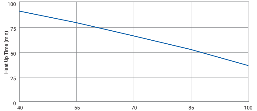
Heat Up Time To 120°F vs Initial Tank Water Temp. @ Ambient Air Temperature 75°F
